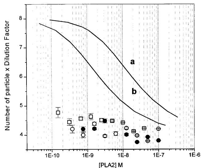
FIGURE 2: Changes of particle number with dilution. Samples of fluorescein-labeled C. atrox PLA 2 have been diluted in the absence (open circles) and in the presence of 10 mM \text{Ca}^{2+} (filled circles) in 50 mM Tris, pH 8. Fluorescein in the same buffer was used as a control (open squares). The number of particles was calculated from the G(0) , and the number of particles multiplied by the dilution factor was plotted against protein concentration (in terms of monomer concentration). For reference, simulation curves are shown for dissociation constants of 36 (a) and 4.3 nM (b).
